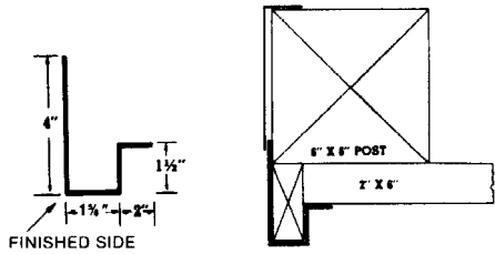
DOOR POST TRIM Number 2930 Color Length White 10'
