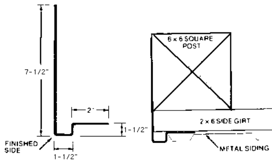
DOOR POST TRIM Number 2930 Color Length White 10'
