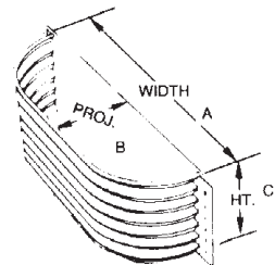
Straight Areawall AWS
