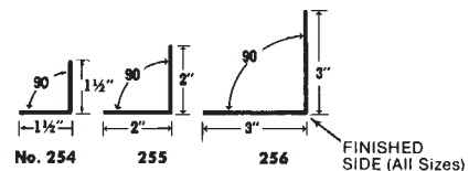
ANGLE TRIM
