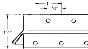
SAW KERF "T" BRACING
