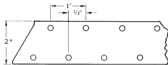
FLAT WALL BRACING
